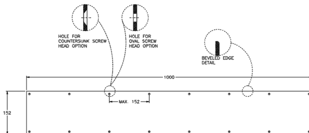
MOP PLATE
