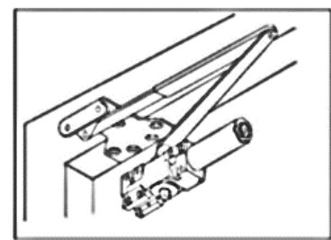
Parallel arm-Push Side
