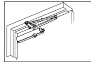
PARALLEL ARM INSTALLATION CLOSER IS INSTALLED ON PUSH SIDE OF DOOR
