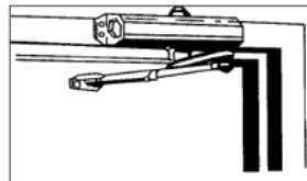
TOP JAMB INSTALLATION CLOSER IS INSTALLED ON FRAME ON PUSH SIDE OF DOOR
