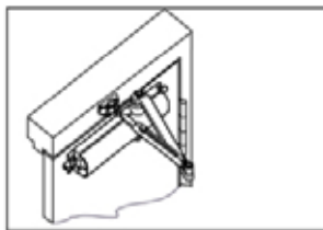
REGULAR ARM INSTALLATION CLOSER IS INSTALLED ON PULL/HINGE SIDE OF DOOR
