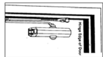
PARALLEL ARM INSTALLATION CLOSER IS INSTALLED ON PUSH SIDE OF DOOR
