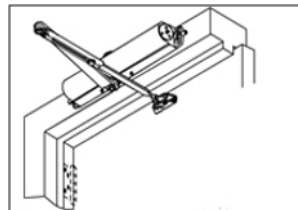
TOP JAMB INSTALLATION CLOSER IS INSTALLED ON FRAME ON PUSH SIDE OF DOOR
